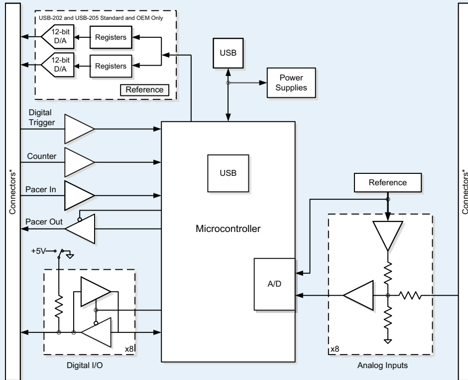
USB-200 Series Block Diagram
